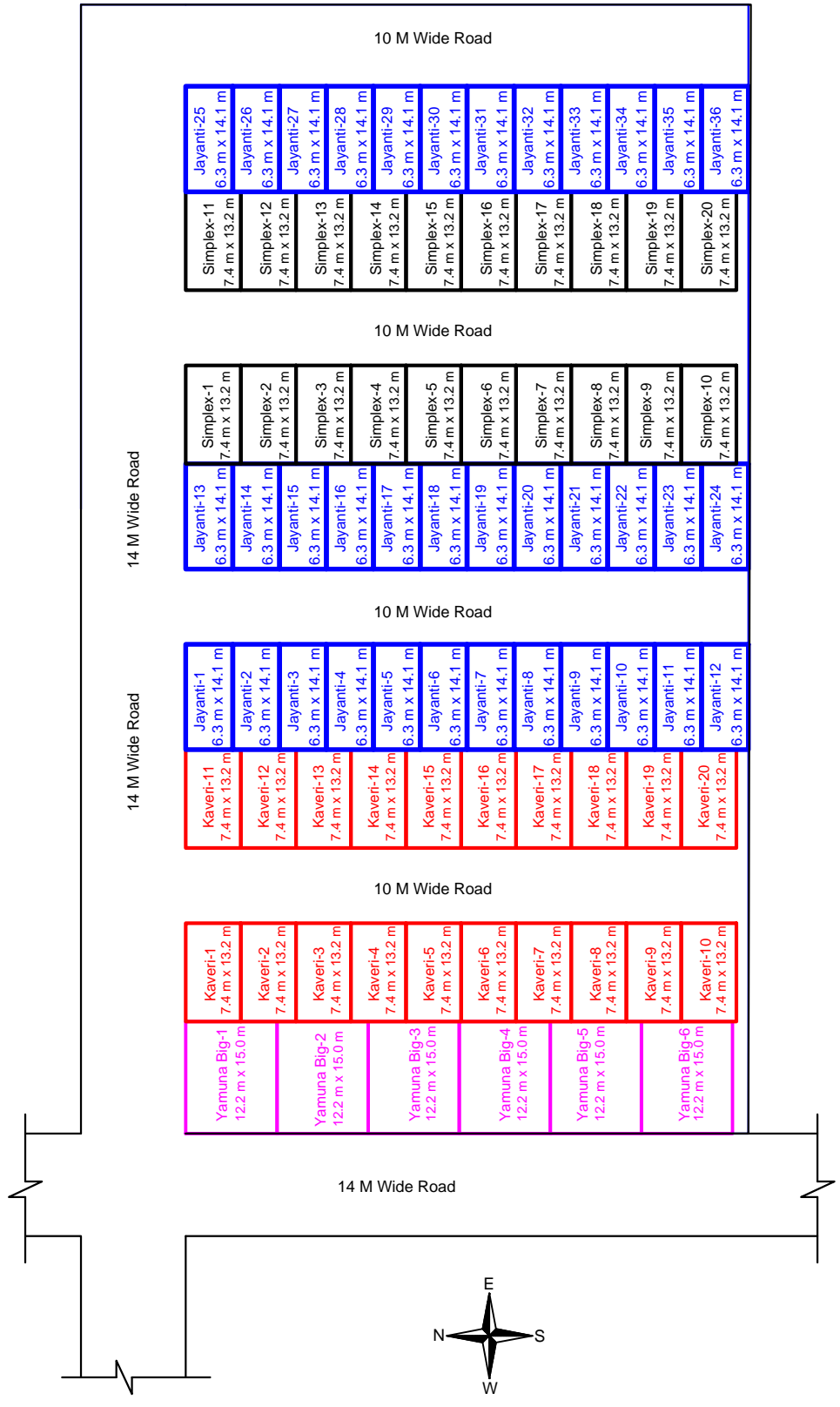
Proposed Site Lay out plan For VASTU VIHAR at Kisan path, Barabanki, Uttar Pradesh
